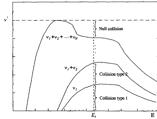
Fig. 2. The addition of the null collision process results in a constant collision frequency over all energies.
